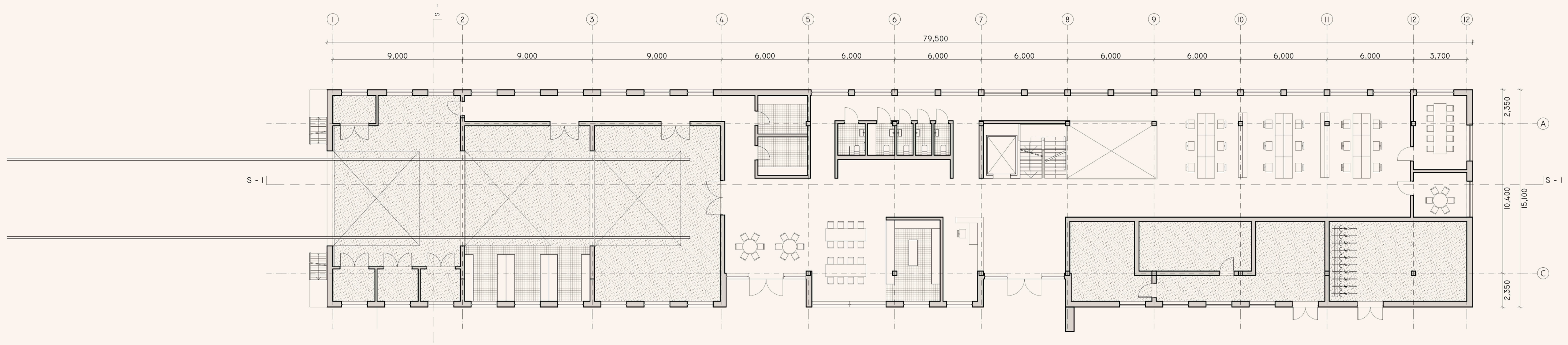
GROUND FLOOR, 1:100
