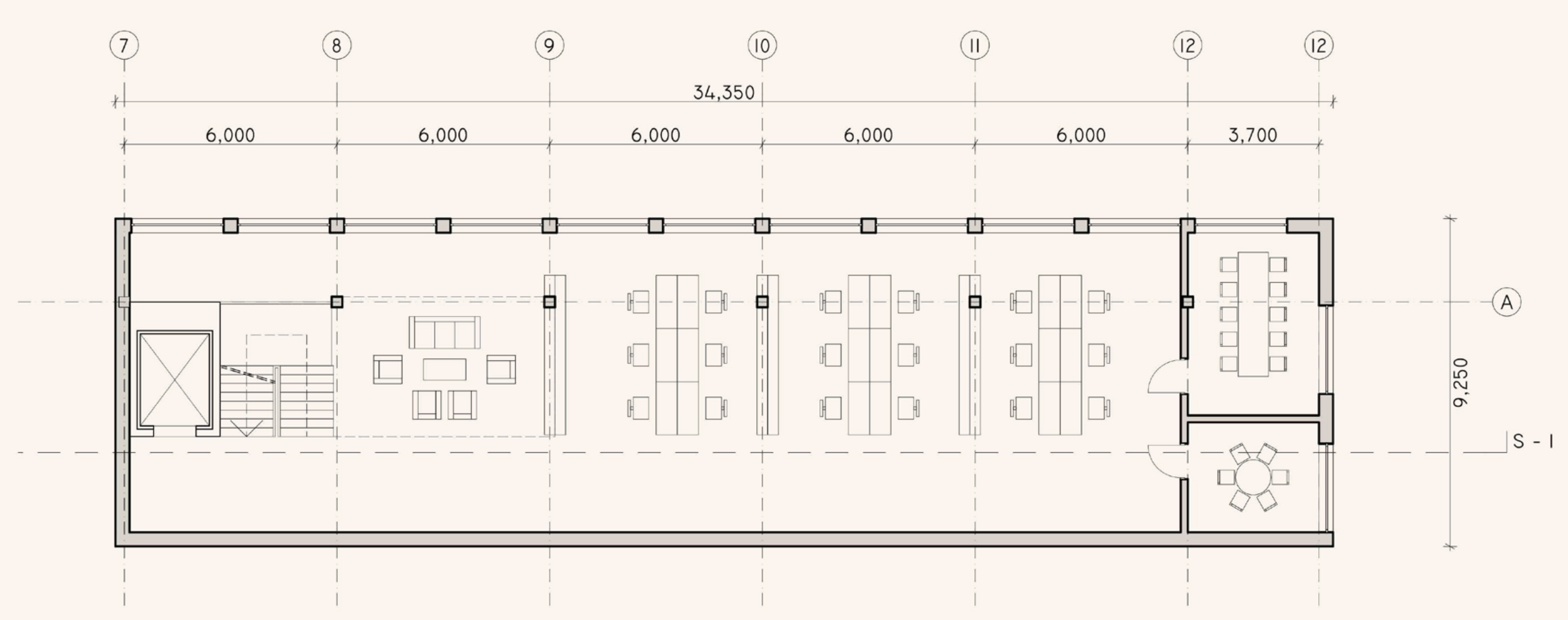
BASEMENT, 1:100
