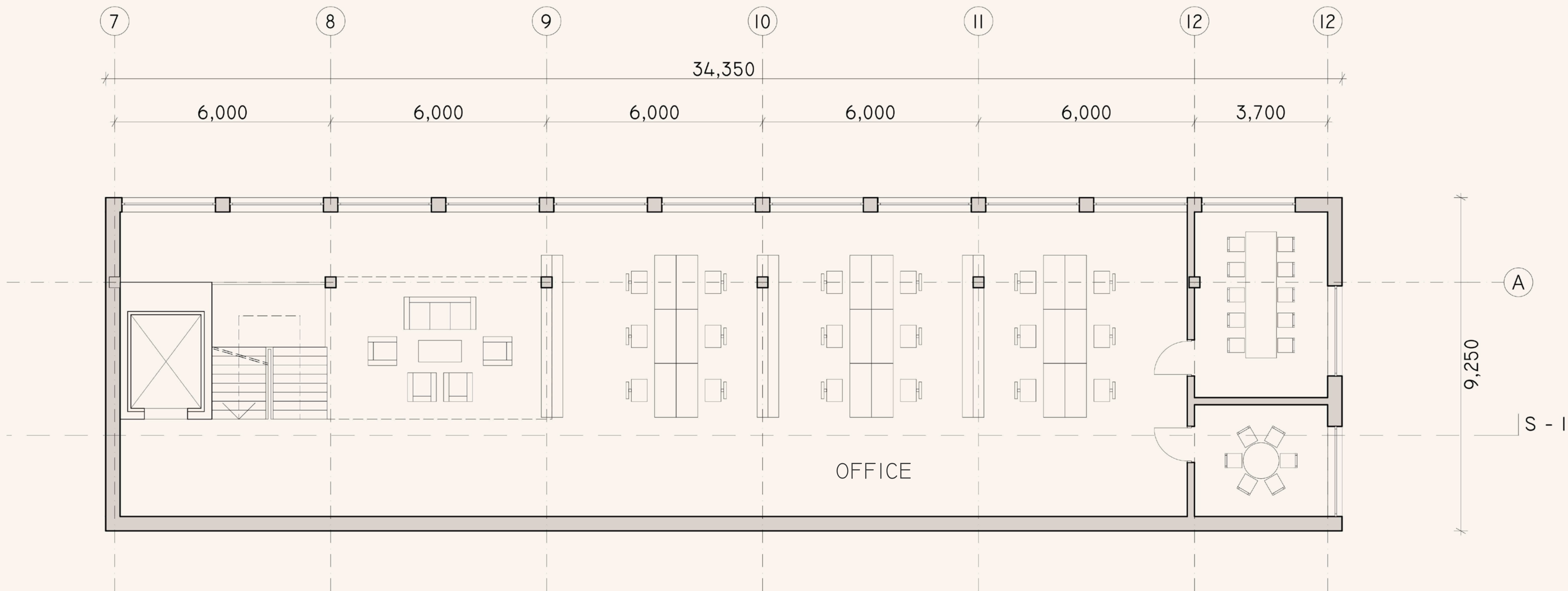
BASEMENT, 1:60
